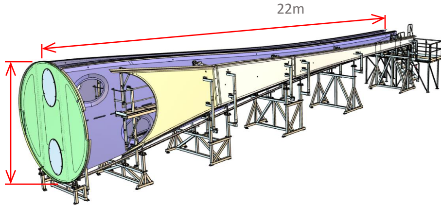
Jig overview, loaded with Webs
