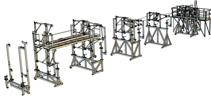
All Jig parts in relative positions, with end platform and intermediate walkways
