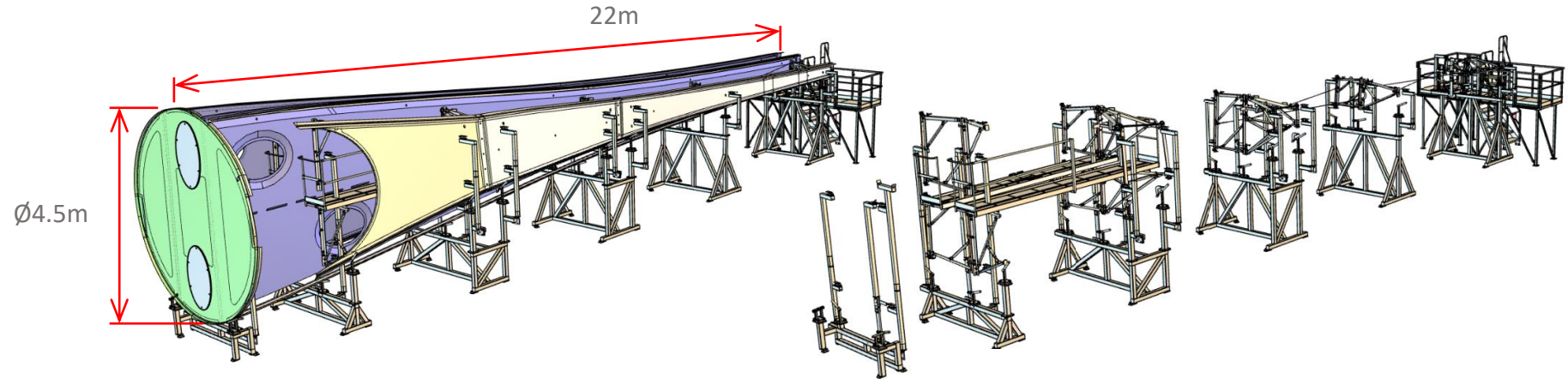
Jig overview, loaded with Webs
