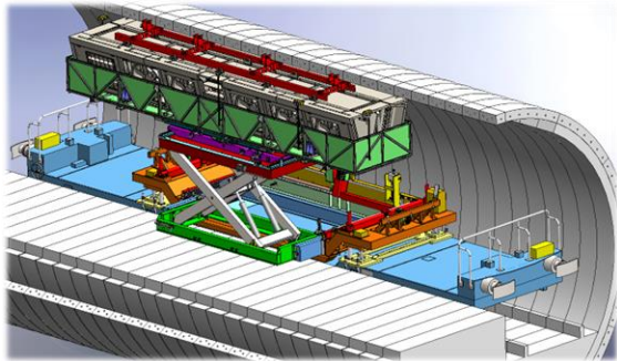
Jig overview, loaded with Webs
